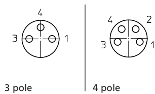
Pin assignments for female M8 connectors, A-coded, front view
